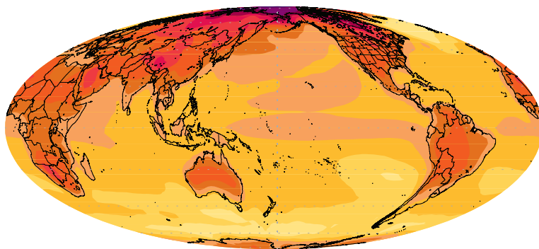
a) Multi-model ensemble 21st Century Change in Temperature (°C/°C Global Warming)
