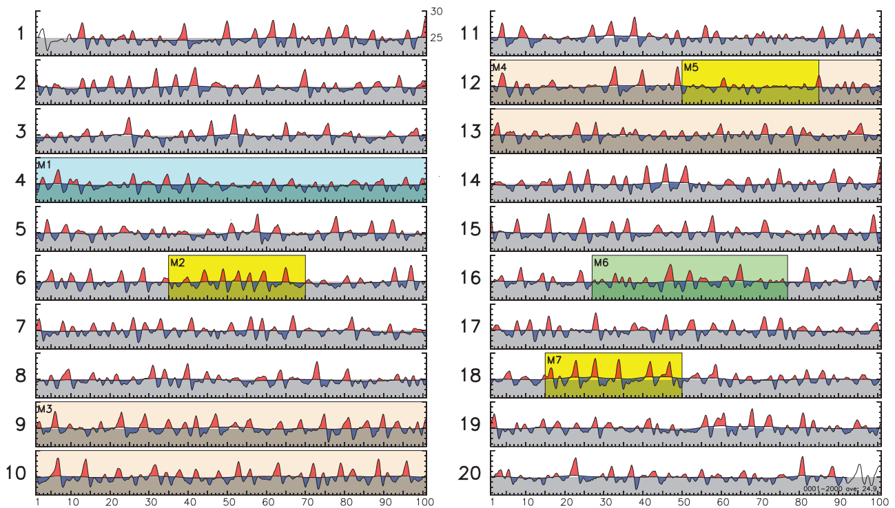
NIÑO3 SST (°C) from 2,000 Years of the GFDL-CM2.1 Preindustrial Control Simulation
