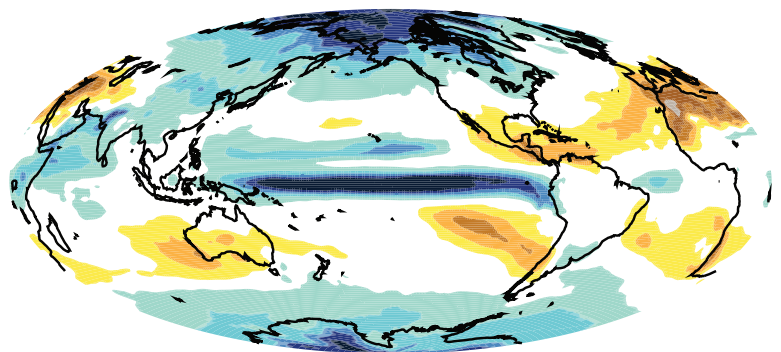
b) Multi-model ensemble 21st Century Change in Precipitation (%/°C Global Warming)
