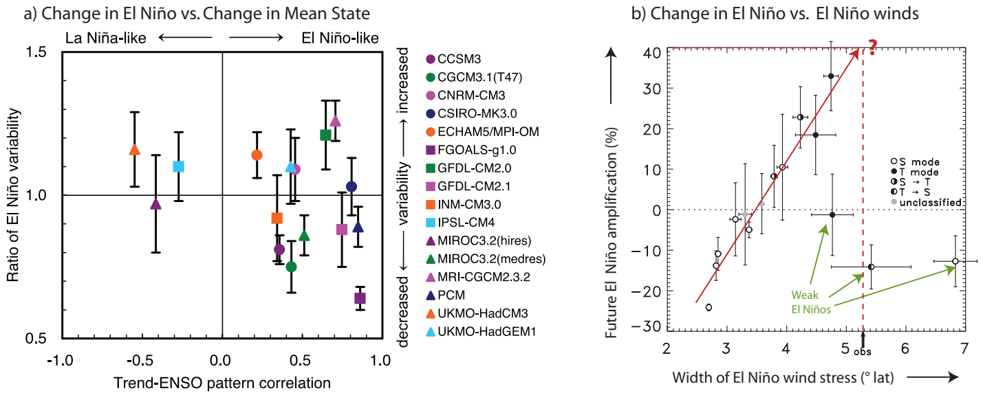
Figure 5: 21st Century projected changes in El Niño characteristics. (a) Multi-model projections of changes in tropical Pacific sea level pressure mean state (horizontal axis) vs. change in El Niño SST variability (vertical axis); the “mean state” change in each model is characterized by its similarity to the pattern of El Niño variability. Changes in mean state and El Niño are computed by comparing the end of the 21st Century projections with the end of the 20th Century from the analysis of Ref. 34. (b) Change in El Niño amplitude (vertical axis) vs. the meridional (northsouth) width of the pre-industrial near-equatorial westerly wind anomalies associated with El Niño, in response to increasing levels of atmospheric CO 2 , from the CMIP3 ensemble of global climate models; different symbols indicate character of model response as characterized in Ref. 27. The three models highlighted by green arrows have 20th Century El Niño variations that are much weaker than observed and are considered less reliable. Left panel adapted from Ref. 43 with permission. Right panel adapted from Ref. 58, copyright American Meteorological Society, reprinted with permission.
