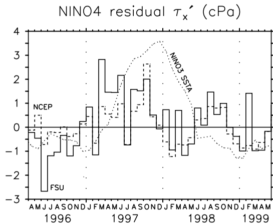
Figure 4: Residual zonal wind stress (cPa) averaged over the NINO4 region ( 160^{\circ}\text{E} – 150^{\circ}\text{W} , 5^{\circ}\text{S} – 5^{\circ}\text{N} ) for FSU (solid) and NCEP (dashed). Also shown are the SST anomalies ( ^{\circ}\text{C} ) averaged over the NINO3 region ( 150^{\circ}\text{W} – 90^{\circ}\text{W} , 5^{\circ}\text{S} – 5^{\circ}\text{N} , dotted).
